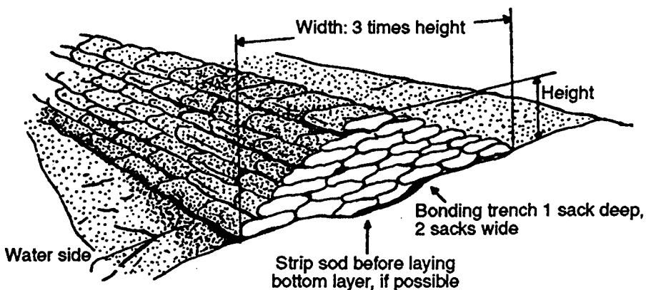
Figure 3. Stacking sandbags.
