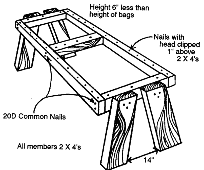
Figure 1. Rack for filling sandbags.
