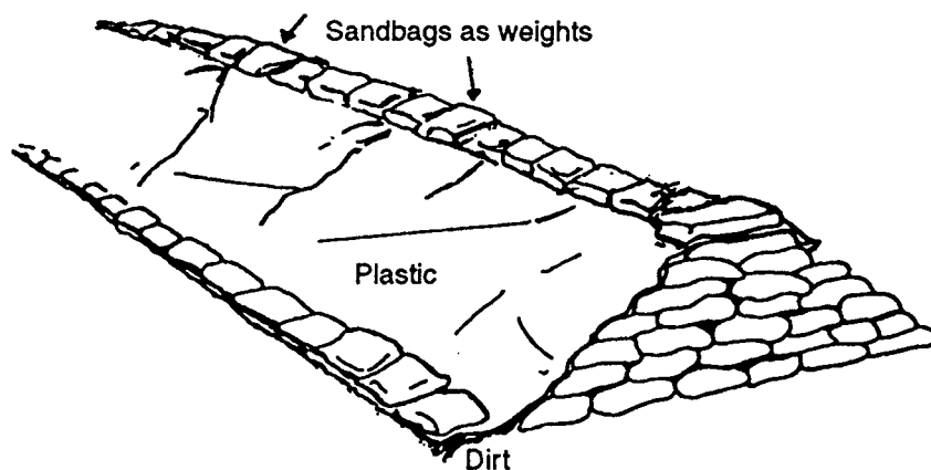
Figure 4. Sealing the sandbag dike.
